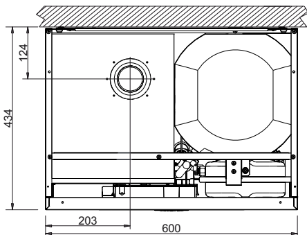
fig. 45- Top view
