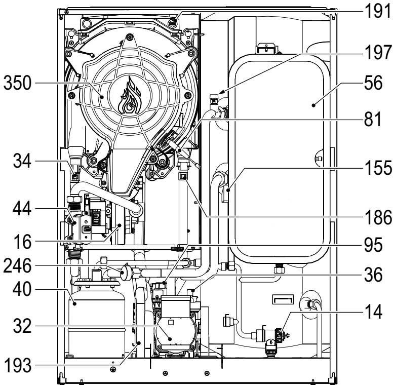
fig. 47- General view
